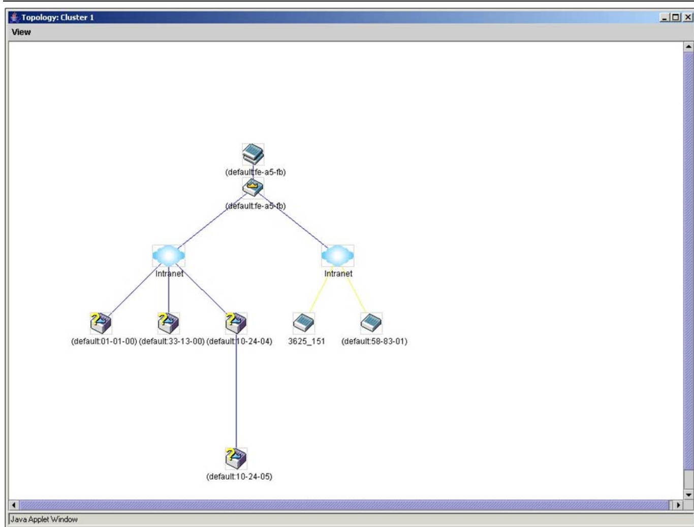
Figure 3-18 Topology view
