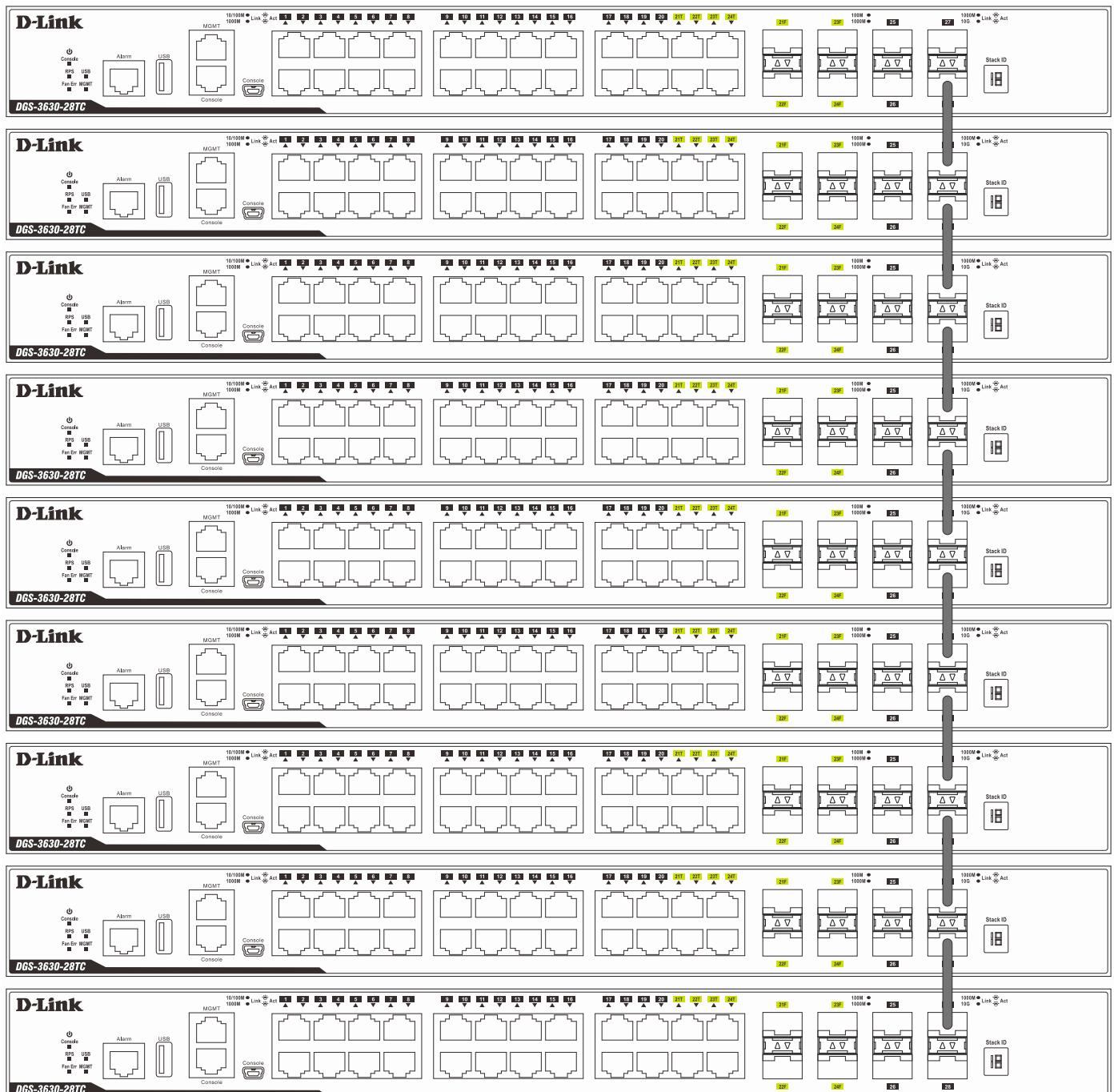
Figure 4-82 Duplex Chain stacking topology (SFP+)
